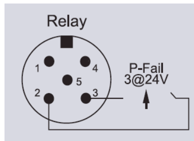
Pin assignment of alarm relay
