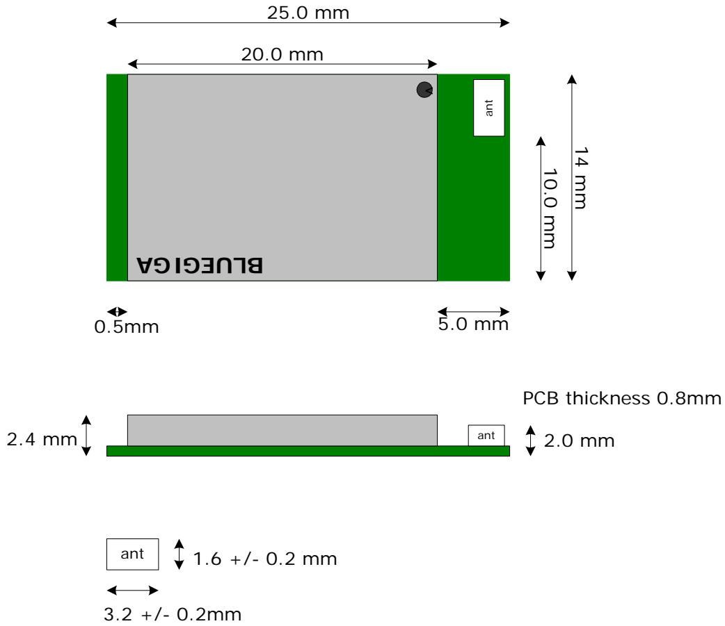
Figure 29: WT12 dimensions
